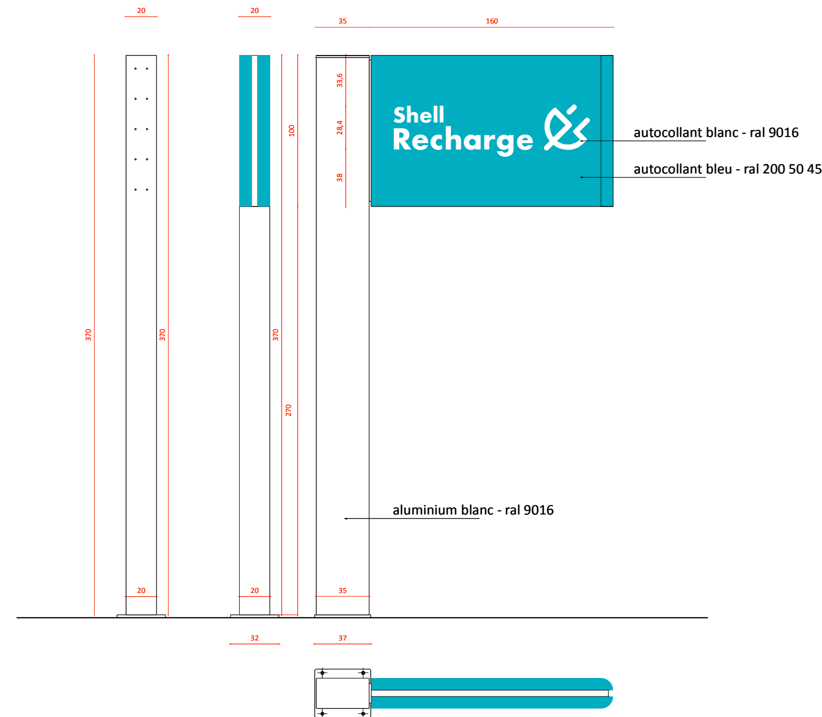
panneau de station de recharge spreader (H: 3,70m)
