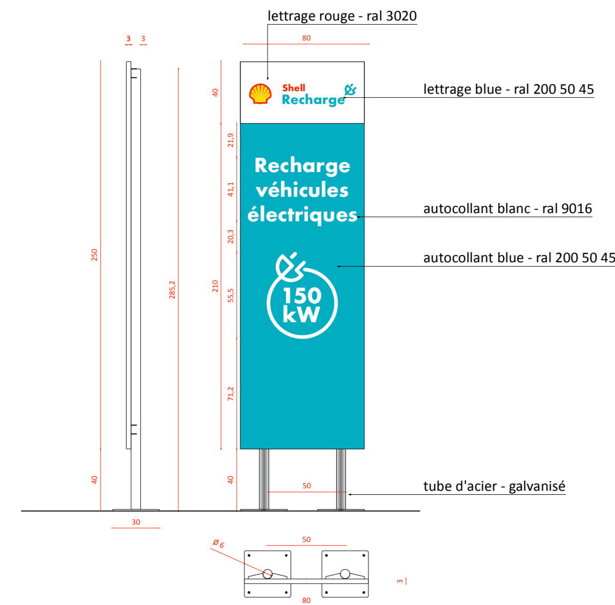
panneau de station de recharge "charging bay sign"
